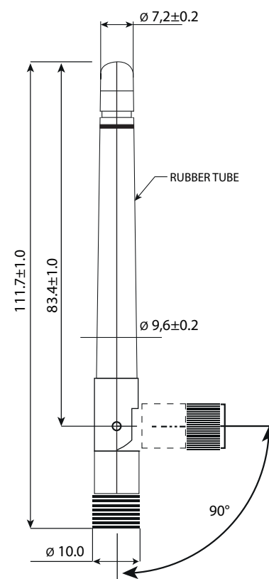
Mechanical Specifications
